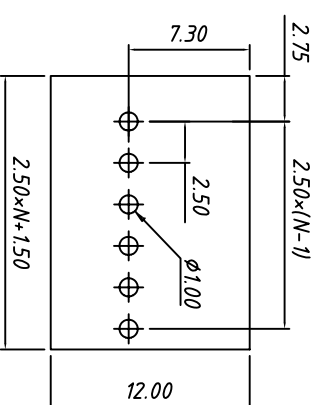
C type PCB LAYOUT
